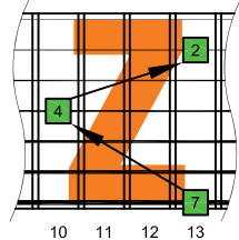
STRING NUMBERS
