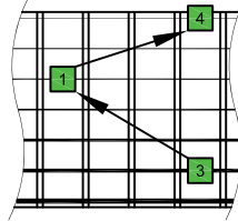
STRING NUMBERS
