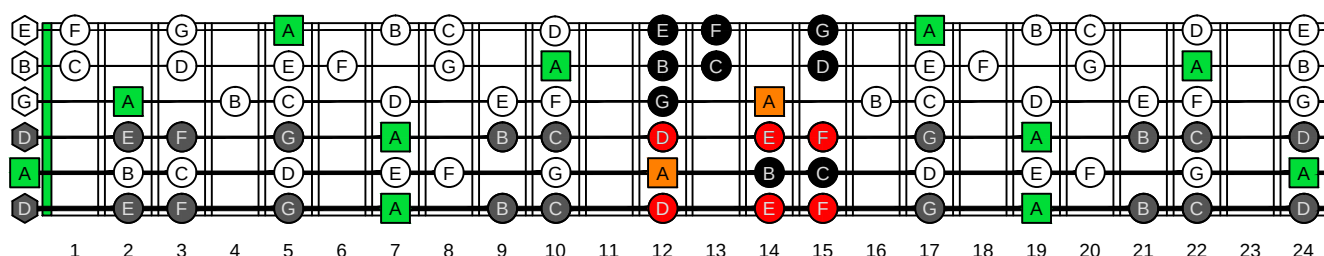
5Am3 at 12 A minor scale (aeolian mode) - ENTIRE FINGERBOARD NOTE NAMES
