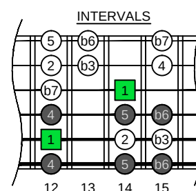
A minor scale SEMITONOMETER
