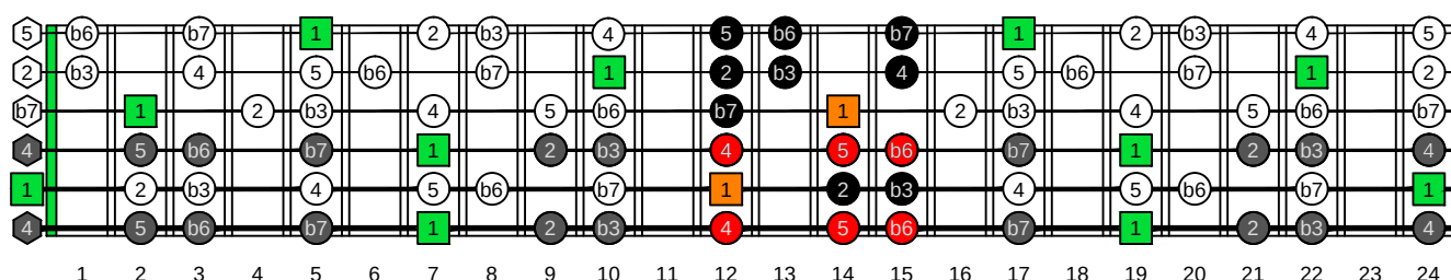
5Am3 at 12 A minor scale (aeolian mode) - ENTIRE FINGERBOARD INTERVALS
