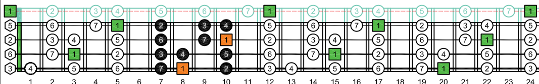
CAGED4BASS 3 notes per string C major scale (Ionian mode) 4E2 box shape : ENTIRE FINGERBOARD INTERVALS
