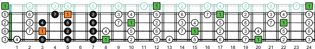
CAGED4BASS 3 notes per string C major scale (Ionian mode) 3A1G box shape : ENTIRE FINGERBOARD INTERVALS
