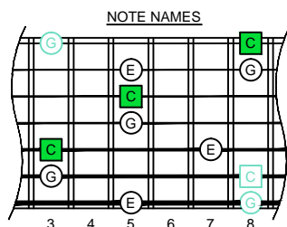
BOX SHAPE
