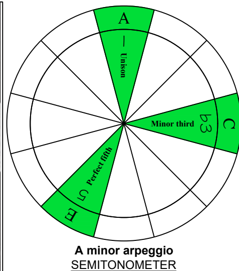
INTERVALS
