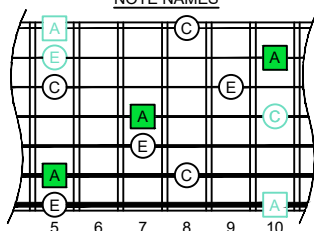
NOTE NAMES
