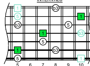
INTERVALS
