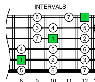
C major scale ( ionian mode ) SEMITONOMETER
