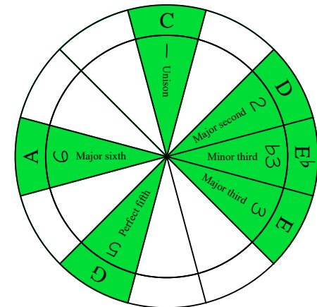
C major blues scale SEMITONOMETER
