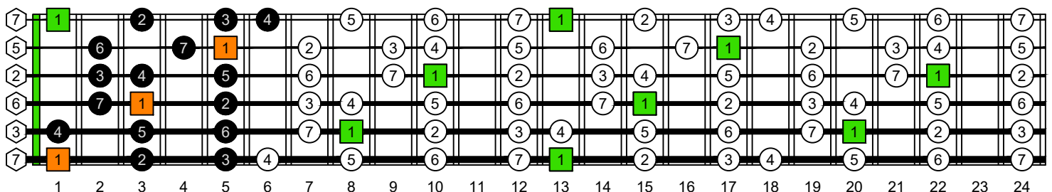
BAGED octaves (6-string guitar : 6/7 ths guitar tuning - B1:E2:A2:D3:G3:B3) C major scale (ionian mode) - INTERVALS : 6B4A2 box shape (3nps)
