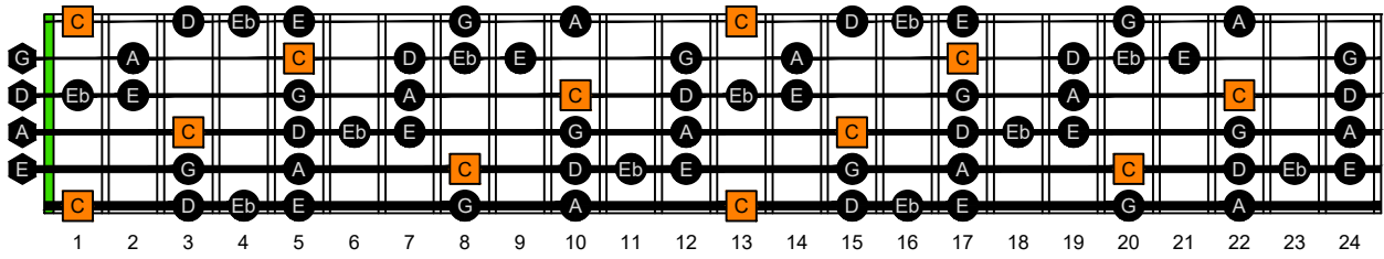
BAGED octaves (6-string guitar : 6/7 ths guitar tuning - B1:E2:A2:D3:G3:B3) C major blues scale - NOTE NAMES : 6B4B1 box shape
