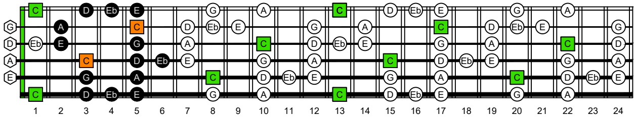
BAGED octaves (6-string guitar : 6/7 ths guitar tuning - B1:E2:A2:D3:G3:B3) C major blues scale - NOTE NAMES : 5G2 box shape
