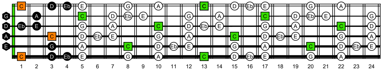
BAGED octaves (6-string guitar : 6/7 ths guitar tuning - B1:E2:A2:D3:G3:B3) C major blues scale - NOTE NAMES : 4A2 box shape
