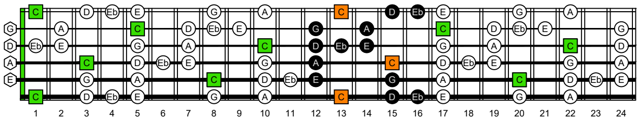
BAGED octaves (6-string guitar : 6/7 ths guitar tuning - B1:E2:A2:D3:G3:B3) C major blues scale - NOTE NAMES : 6B4B1 box shape at 12
