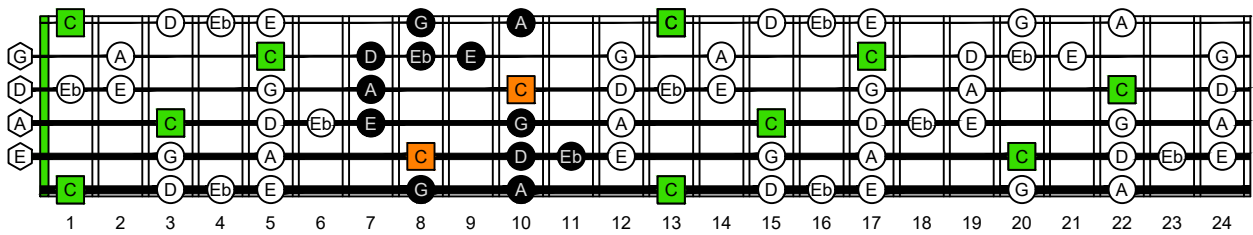
BAGED octaves (6-string guitar : 6/7 ths guitar tuning - B1:E2:A2:D3:G3:B3) C major blues scale - NOTE NAMES : 6D3D1 box shape
