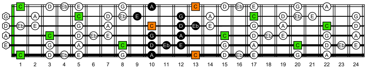
BAGED octaves (6-string guitar : 6/7 ths guitar tuning - B1:E2:A2:D3:G3:B3) C major blues scale - NOTE NAMES : 6B4B1 box shape at 12
