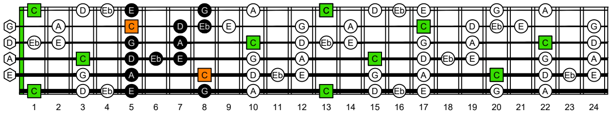
BAGED octaves (6-string guitar : 6/7 ths guitar tuning - B1:E2:A2:D3:G3:B3) C major blues scale - NOTE NAMES : 5E3 box shape
